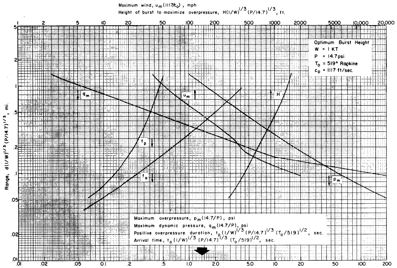
Fig. 2.9—Scaled blast parameters for optimum heights of burst as a function of scaled range. These are plots of Eqs. 2.60, 2.62, 2.64, 2.66, 2.70, 2.74, 2.76, and 2.79 given in Table 2.9.
